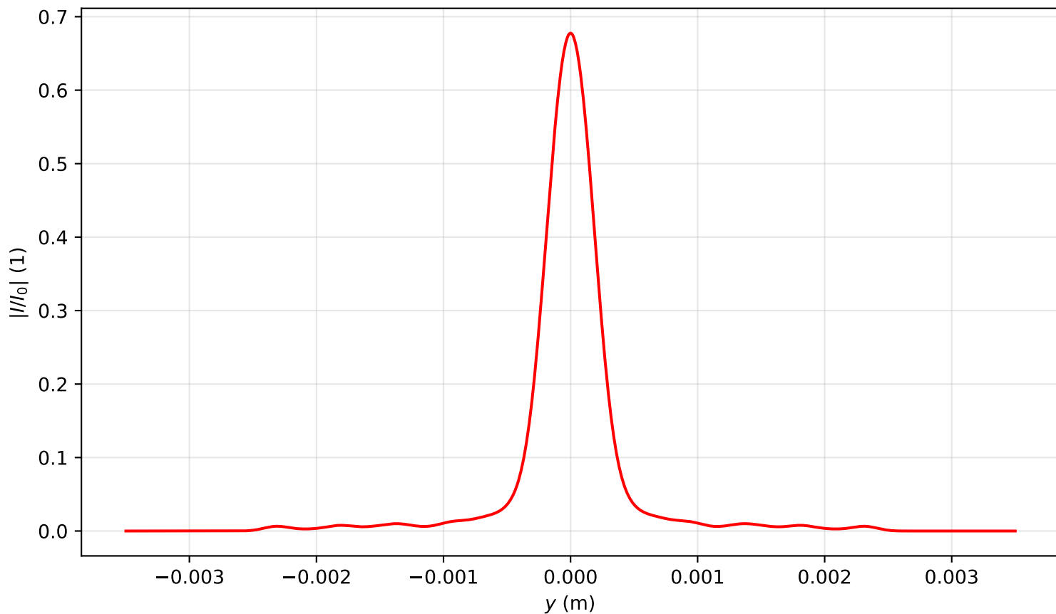
Intensity profile I(x = 0, y, z = 3.503)/I_0 , P_{in}=3.0P_{cr} , artificial time
